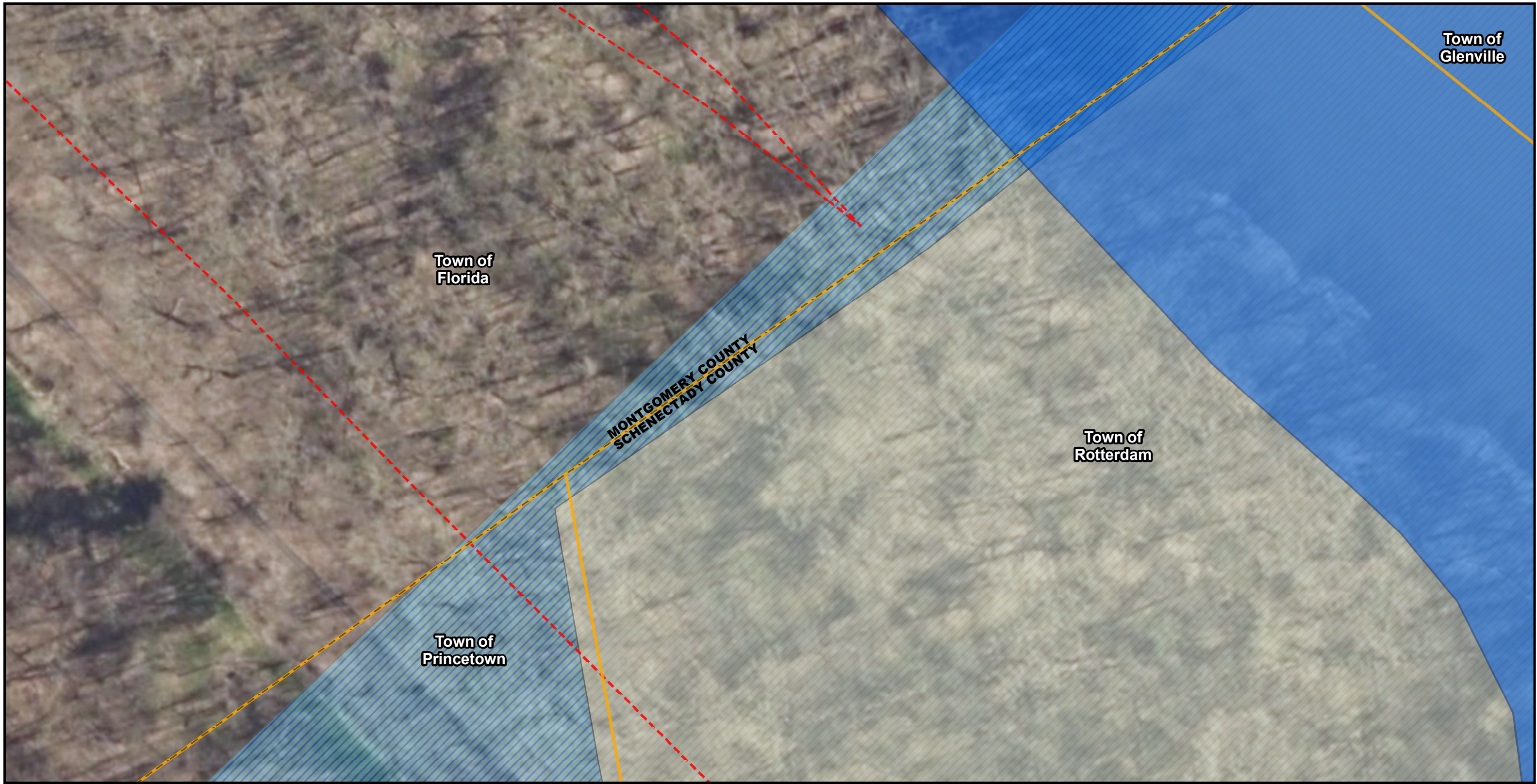
Figure 26F: Aquifers
